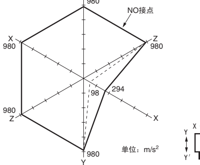
误动作冲击
