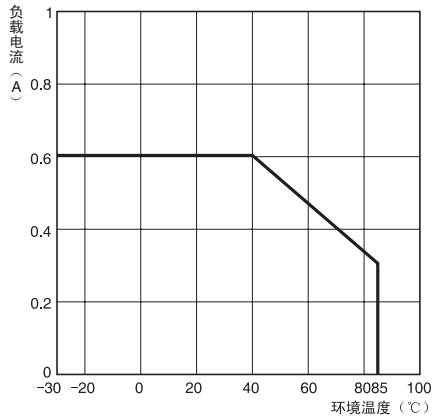
G3DZ-2R6PL
