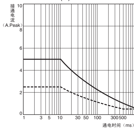
G3DZ-1R5PL(G)
