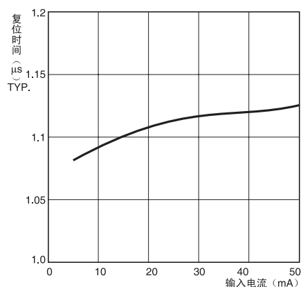
G3DZ-DZ02PG
