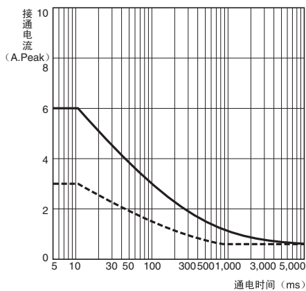
G3DZ-2R6PL
