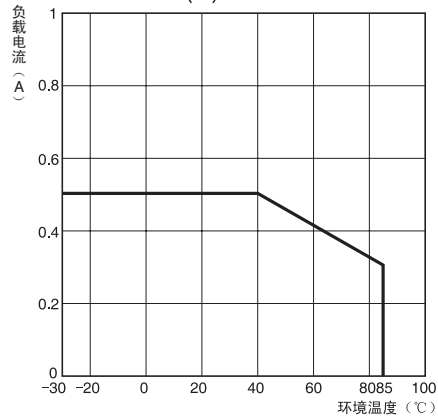
G3DZ-1R5PL(G)
